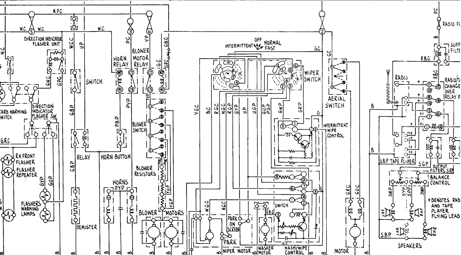
HAZARD WARNING REAR WINDOW DEMISTER HORNS BLOWER MOTORS WINDSCREEN WIPER (INCLUDING INTERMITTENT OPERATION) AND WASHER AERIAL RADIO AND TAPE PLAYER STEREO RADIO STEREO TAPE
