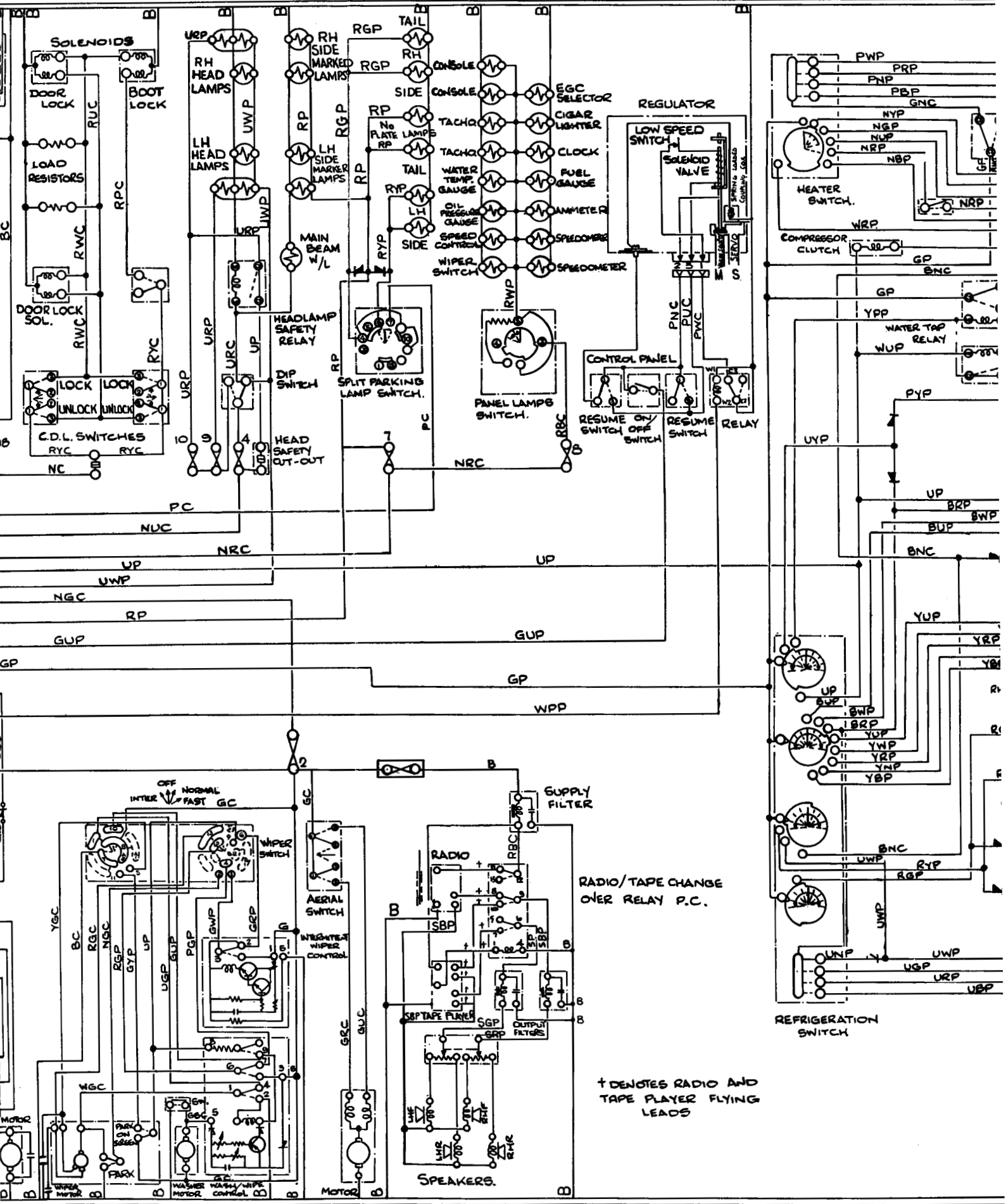
WIPERS WINDSCREEN WIPER & WASHER (INCLUDING INTERMITTENT OPERATION)
