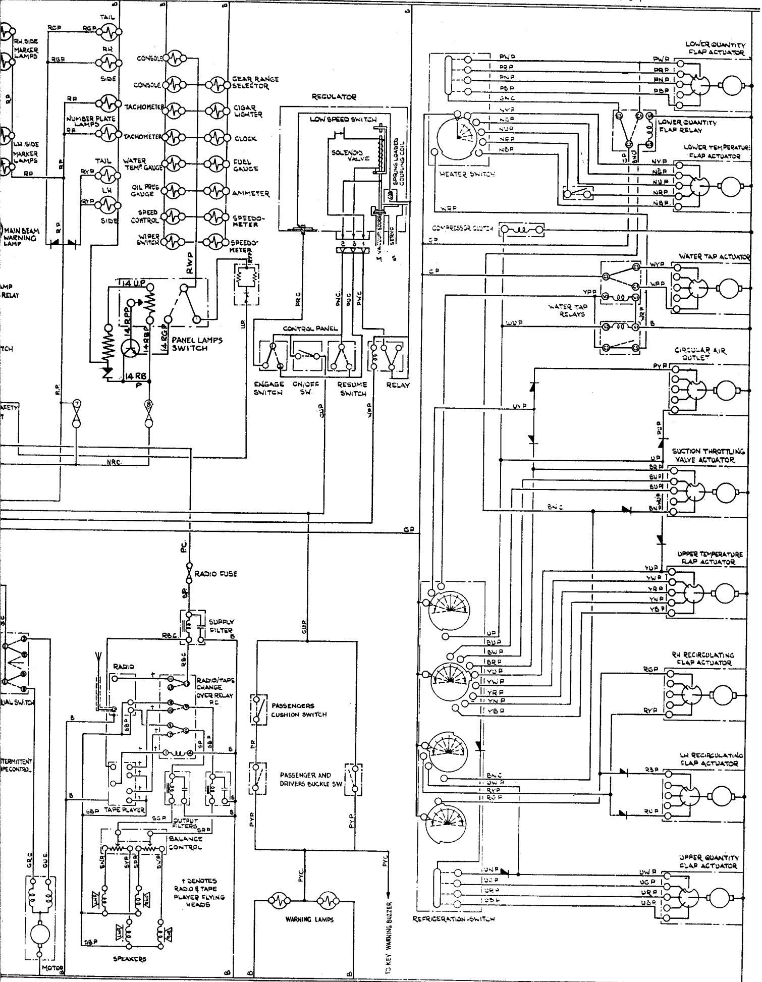
AERIAL RADIO AND TAPE PLAYER - BOTH STEREO
