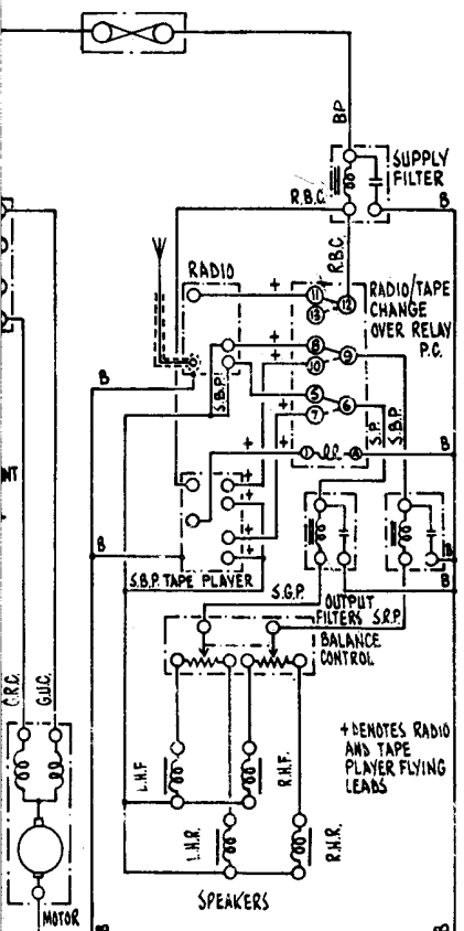
RADIO AND TAPE PLAYER STEREO RADIO/STEREO TAPE
