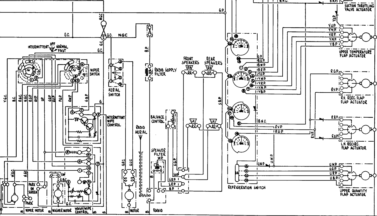
WINDSCREEN WIPER (INCLUDING INTERMITTENT OPERATION) AND WASHER
