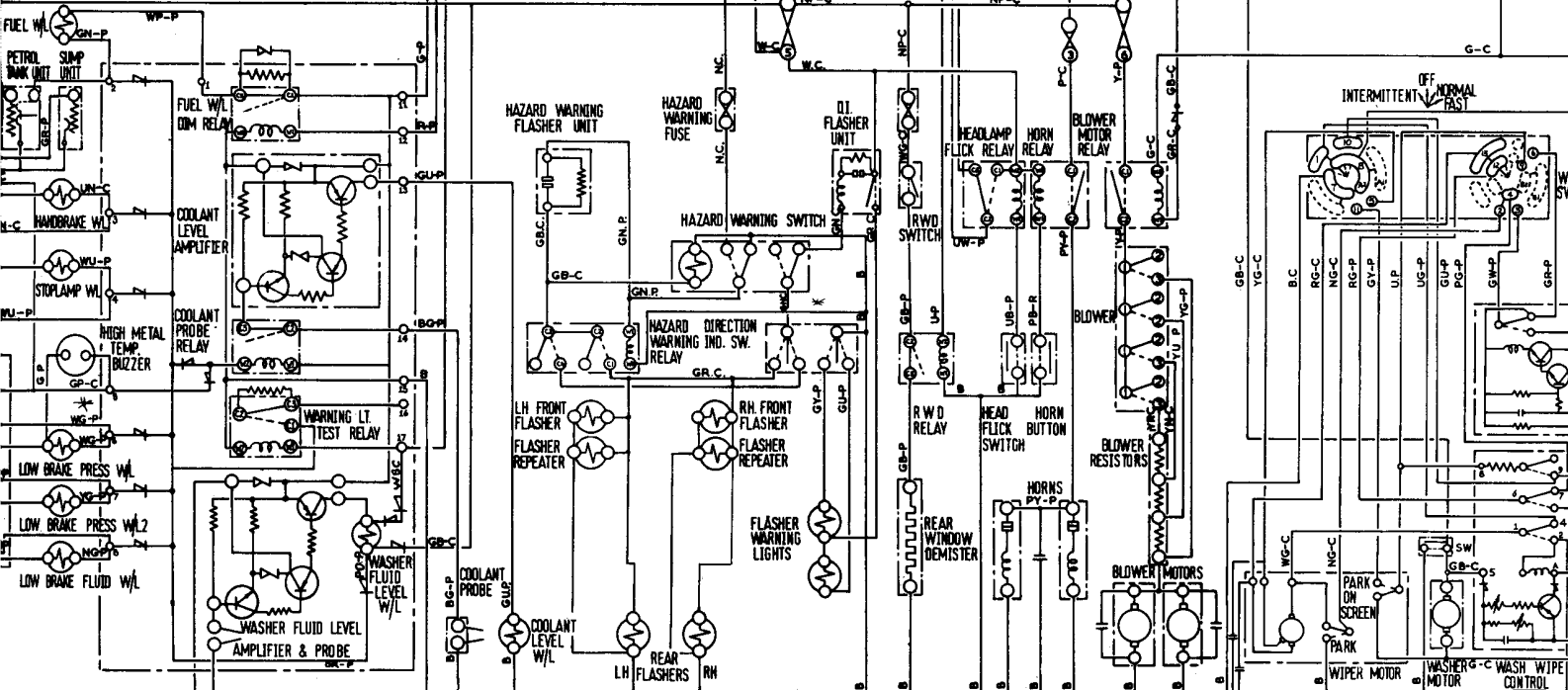
HEADLAMP, WARNING LIGHTS, FUEL GAUGE, HIGH METAL TEMPERATURE BUZZER, COOLANT PROBE.
