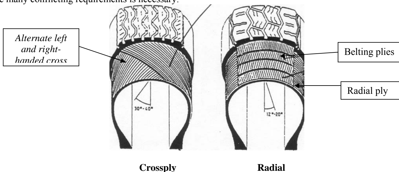
Figure 1. Tyre carcass construction.
