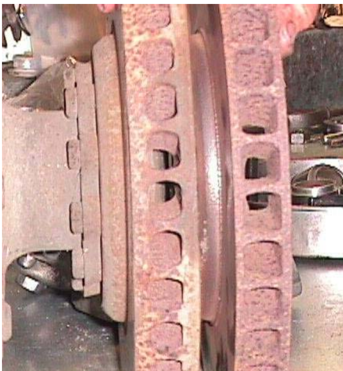
An appalling piece of maintenance. The brake rotor on the right has been ground way beyond the minimum permitted. The rotor on the left is of original dimension
