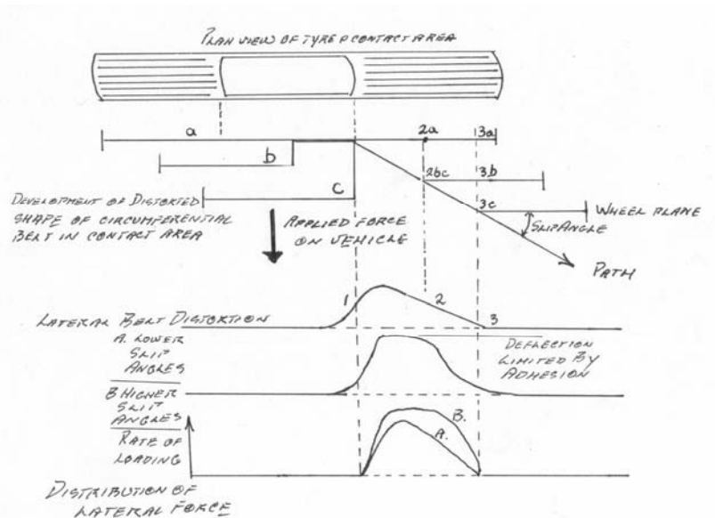
Fig. 4 Exaggerated diagram showing the behavior of a pneumatic tyre when cornering.
