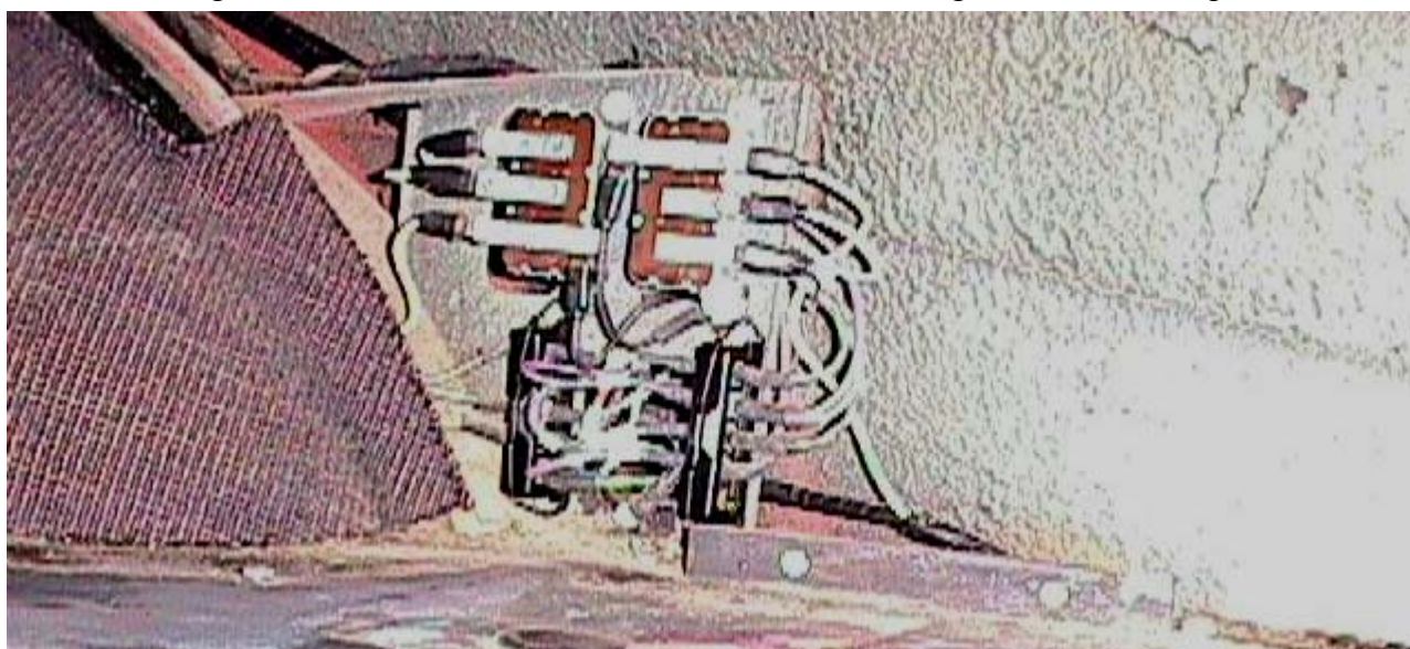
The flasher relays for the tail lights fitted to an S2 and normally hidden behind the right hand boot liner
